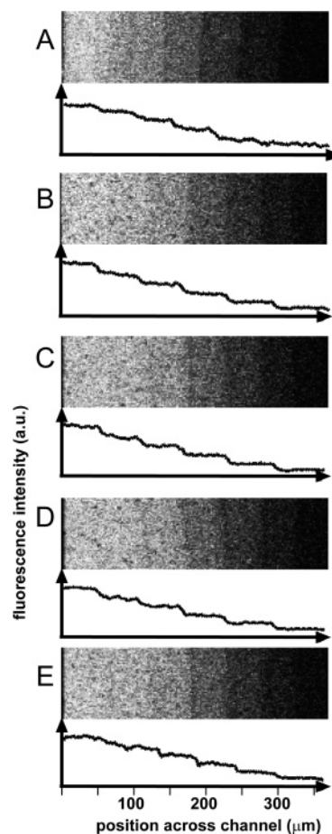
Figure 5. Gradients of various molecules on oxidized PDMS generated by using the avidin–biotin approach. (A) The avidin gradient; (B) a gradient of biotin–fluorescein; (C) a gradient of the 28-mer monobiotinylated DNA; (D) a gradient of biotinylated dextran. (E) A gradient of poly(L-lysine) is made by direct adsorption from a gradient of poly(L-lysine) in solutions. The profiles of the gradients are documented at the bottom of each graph. Light areas corresponds to high surface densities of immobilized molecules.
