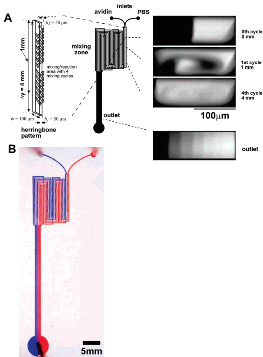
Figure 2. Design of the microfluidic channel that incorporates CAMs. (A) Diffusive mixing is enhanced by chaotic advection generated by an asymmetric herringbone pattern in the ceiling of the microchannels. Visualizations of the flow before entering the chaotic mixer, after the first cycle and after the fourth cycle of the mixer, are given on the right side of the figure. Cross-sectional images were taken with a confocal microscope. The last image (outlet) was compressed by 1/7 in the horizontal axis. The stretching and folding of the flow were visualized by injecting nonfluorescent and fluorescent solutions (avidin, labeled with fluorescein) in the network. A magnified figure that shows the design of the \mu FN is in Figure 3. (B) A photograph of a microfluidic network we used for the immobilization of protein gradients. We used blue and red ink to visualize the channels and illustrate the function of the network and its formation.
