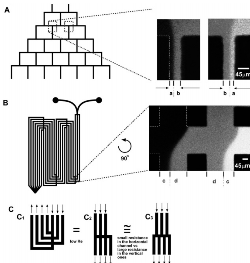
Figure 3. Design of the fluidic network described in this paper. (B) carries out mixing and splitting the same way as the ones in our previous work (A). 1 (A) A schematic diagram of the design for the gradient mixer used in prior work. The micrograph on the right shows the way different streams are split. (B) The micrograph on the right shows that the design used in this paper achieves splitting equivalent to that in (A). Note that the ratios of the widths of the two streams are the same in these designs ( a/b = c/d ). (C) A side-by-side comparison between the two designs: (C1) illustrates the design in (B), while (C3) illustrates the design in (A). For fluids at low Reynolds numbers ( Re < 0.005 in all experiments described in this paper), (C1) is equivalent to (C2). Because the fluidic resistance of the horizontal part of the channel is <5\% of the resistance of the vertical part of the channel, (C2) approximates (C3). Arrows indicate the directions of flow.
