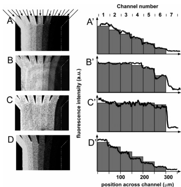
Figure 4. Gradients of immobilized avidin on the surface. Immobilized gradients of avidin generated from gradients of {avidin ↔ PBS} in solution for (A) 5, (B) 15, or (C) 50 min. (D) Immobilized gradients of avidin generated from gradients of {avidin ↔ BSA} in solution for 50 min. (A'), (B'), (C'), and (D') indicate the corresponding measured profiles of intensities of fluorescence across the channels. The vertical columns indicate the theoretical fluorescent intensities (see the section Simulation of Adsorption of Proteins for details) in each channel. See text for details.
