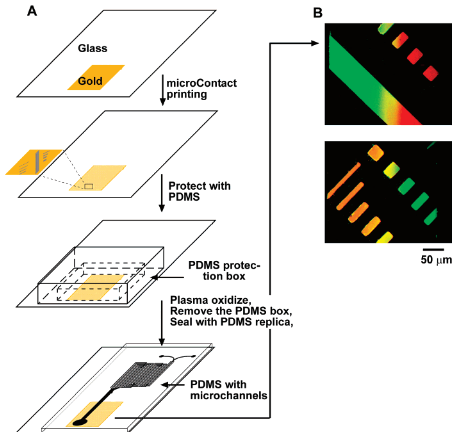
Figure 7. Fabrication of gradients confined in micropatterns. (A) Outline of the fabrication of gradients confined in micropatterns. (B) Fluorescent micrographs of micropatterns that have gradients of laminin (stained green) and fibronectin (stained red) across them.
