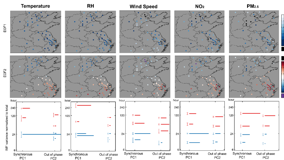
840 Figure 8. EOF-EEMD-HT-MSA results for the observed temperature, RH, wind speed, NO 2 and PM 2.5 . The first two rows depict EOF1 and EOF2, and the third row shows the EEMD-HT-MSA result for PC1 and PC2. In each panel of the third row, the length of the vertical “error bar” shows the RPR of an IMF, while the length of the horizontal bar represents the percentage contribution of the IMF to the total variance of the original data (as such, the horizontal lengths for different IMFs across different PCs can be compared). The blue (red) color indicates diurnal (day-to-day) variation.
